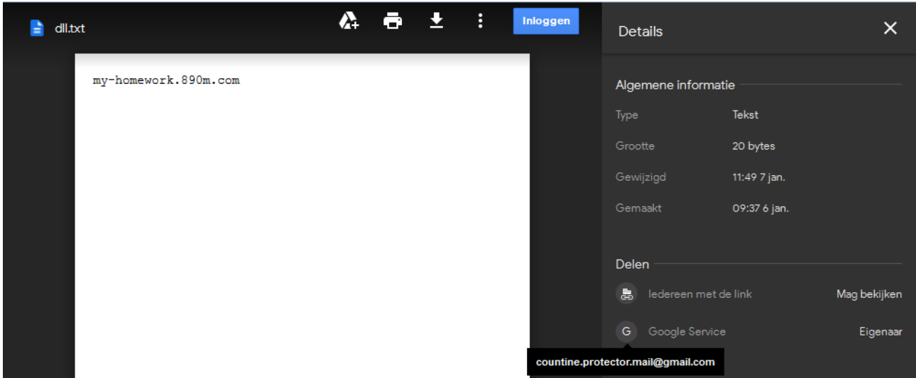
Figure 4. File stored in the attacker’s Google Drive
