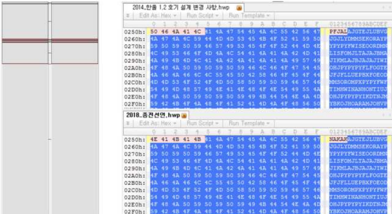
Figure 10. Shellcodes of the malicious files from 2014 (top) and 2018 (bottom)
